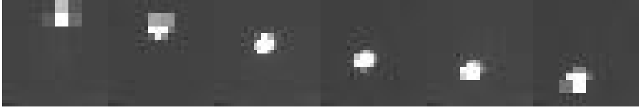
Figure 3-5(b) Six frames taken of a focused moving laser spot with the variable acuity sensor was operating with a high spatial resolution foveal region in the center of the array.
