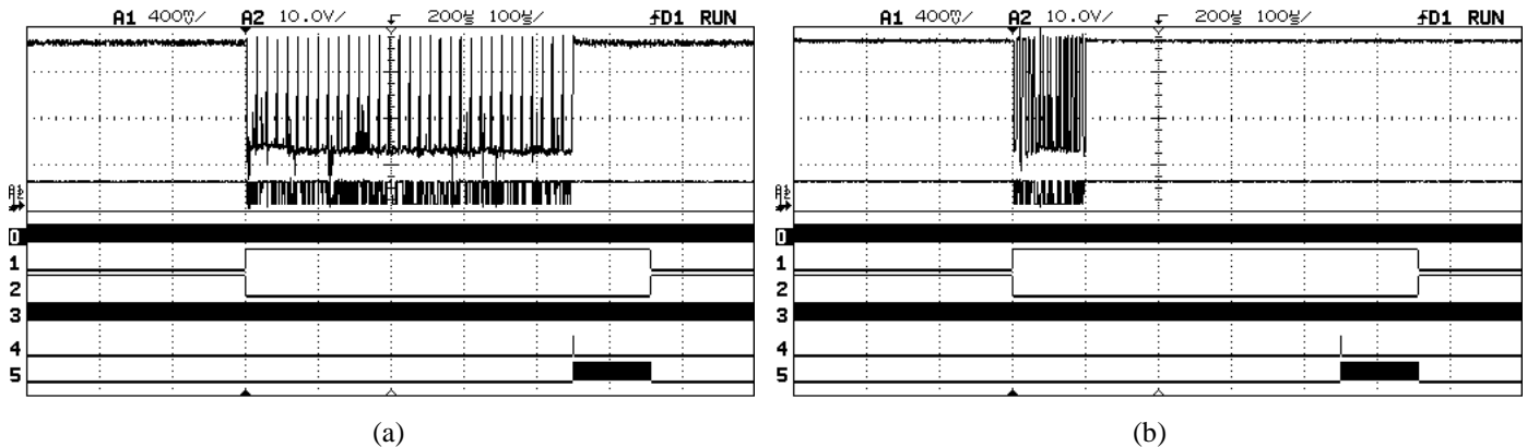
Figure 3-1 Oscilloscope waveforms of one readout frame in both non-superpixel configuration (a) and 4x4 superpixel configuration (b) showing analog pixel output trace (top) and digital output trace, and the input clocks (0-5). Note that in superpixel configuration only one-fourth of the pixel values are multiplexed off-chip, allowing for an increased frame rate.
